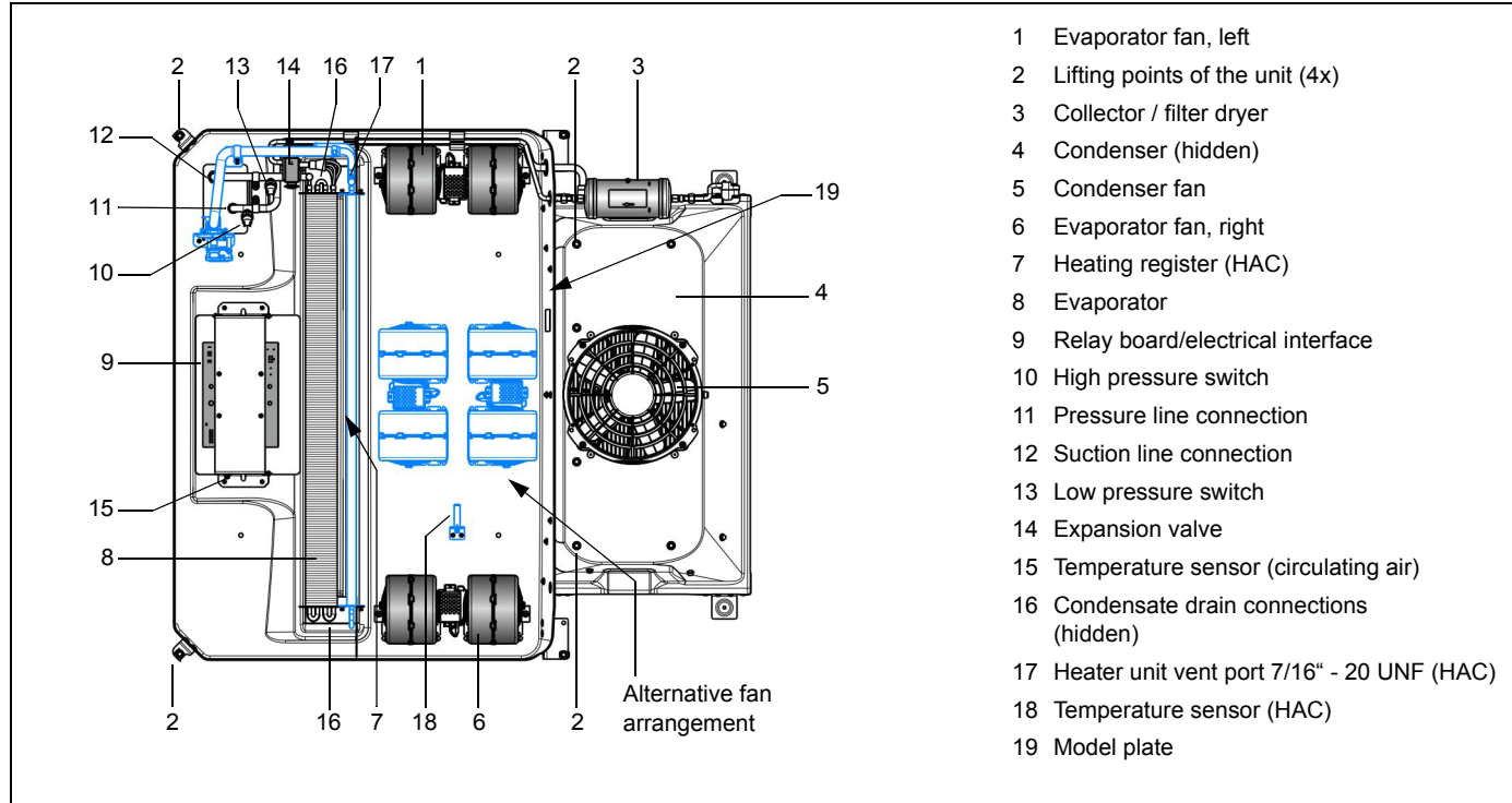
Fig. 1: Minisphere 100 AC/HAC
