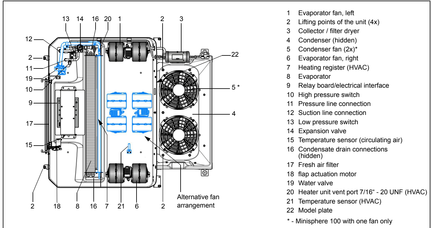
Fig. 3: Minisphere 100/130 VAC/HVAC
