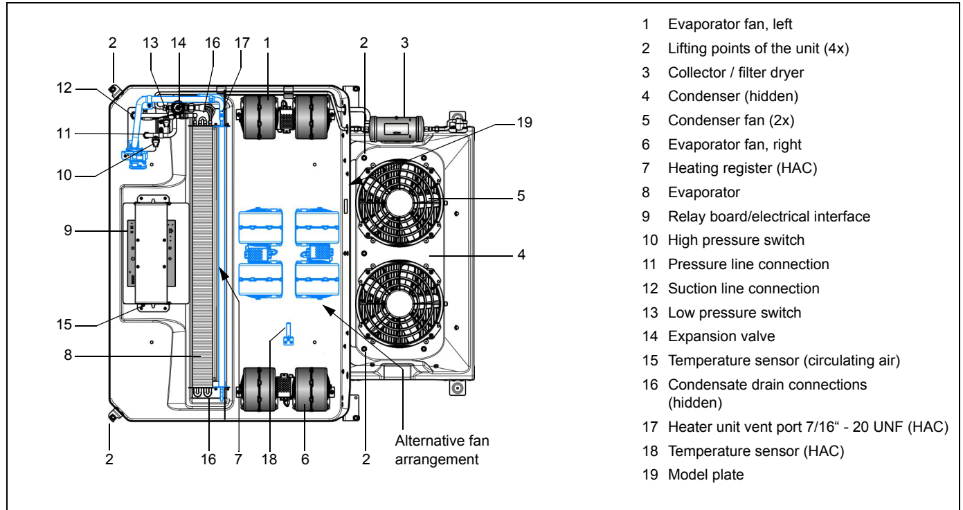
Fig. 2: Minisphere 130 AC/HAC
